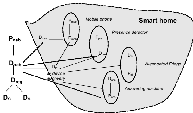
Fig. 3. The Nabaztag joining a Smart Home.
