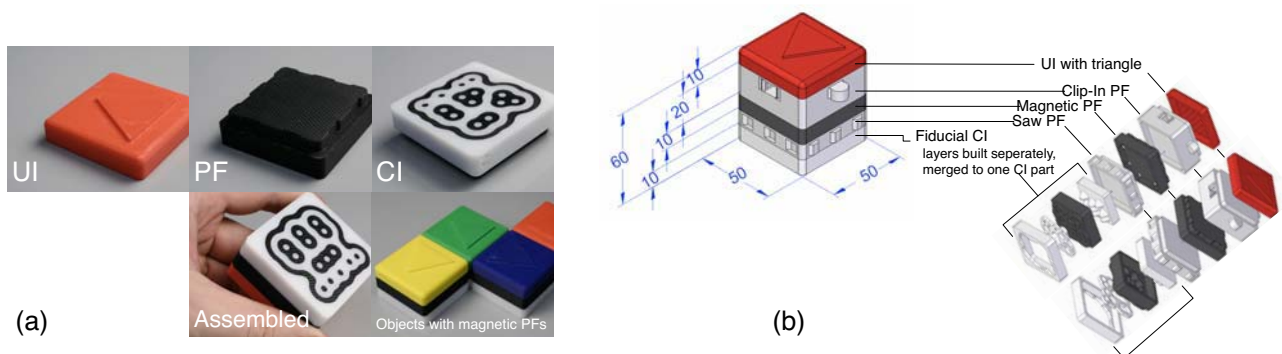
Figure 1. Design and implementation of TUImod elements. (a) TUImod modular design. (b) TUImod object with all PF elements covered by example elements for UI and CI. Left – Assembly, Right – Explosion view.
