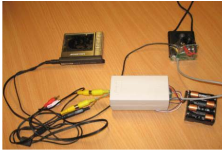
Figure 3: SenseCam with video logging hardware
